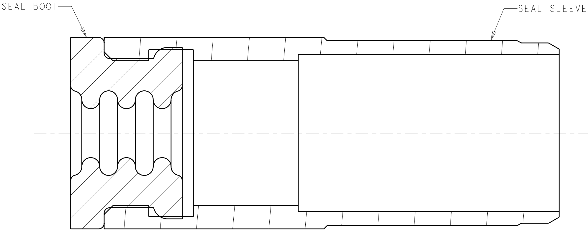
SECTION J-J
