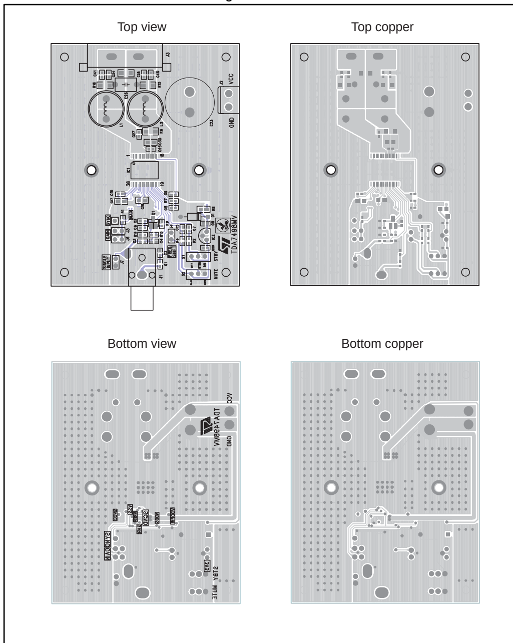
Figure 3: Test board
