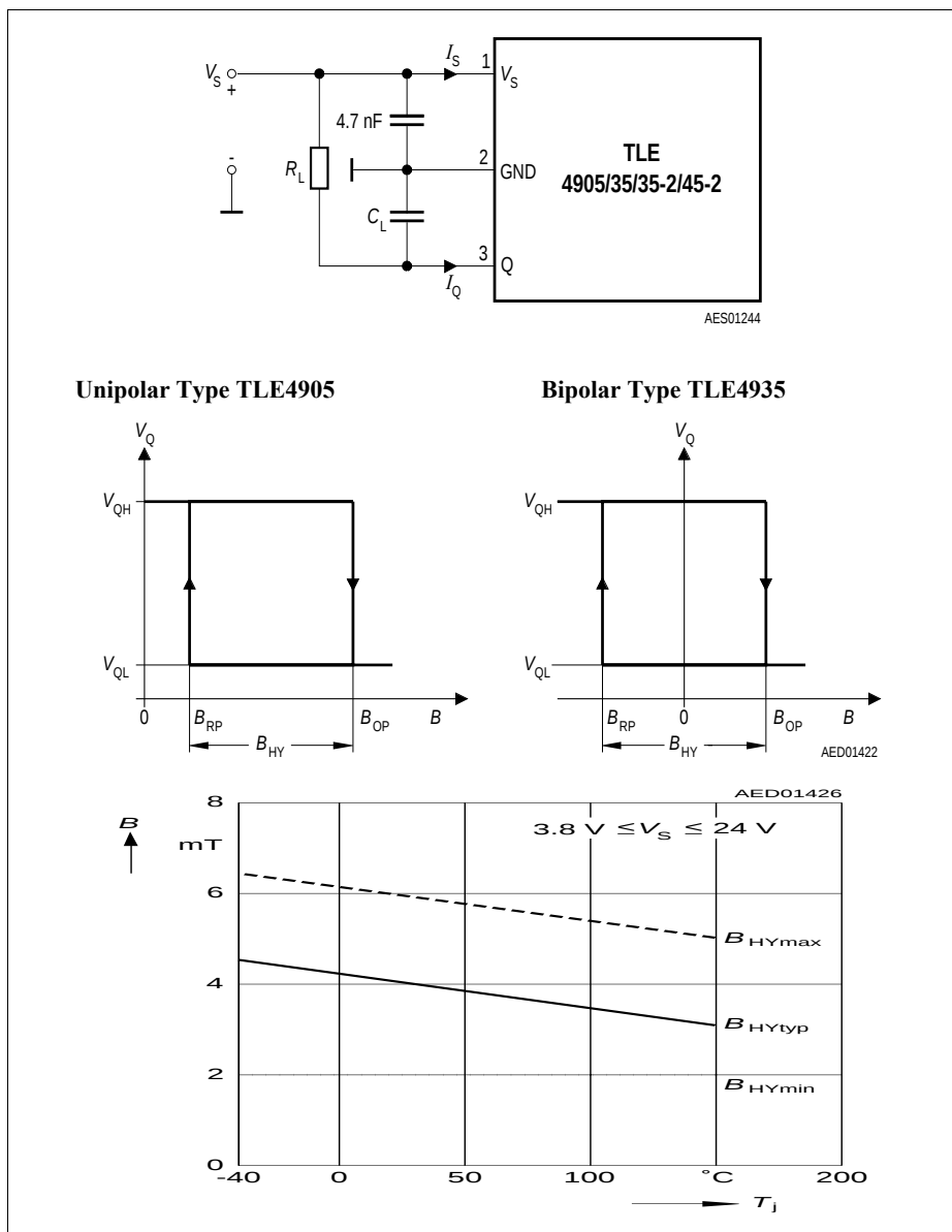
Figure 7 Test Circuit 1
