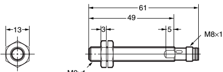
E2A-S08LS02-M5-□□
