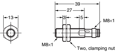
E2A-S08KS02-M5-□□
