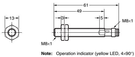
E2A-S08LS02-M5-□□
