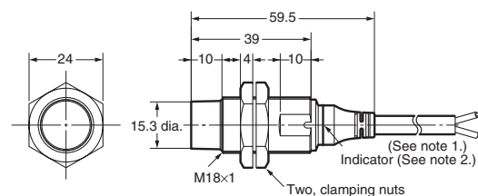
E2A-M18KN16-WP-□□
