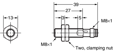
E2A-S08KS02-M5-□□
