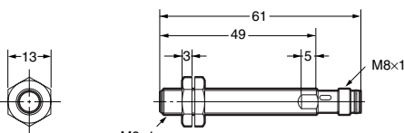
E2A-S08LS02-M5-□□
