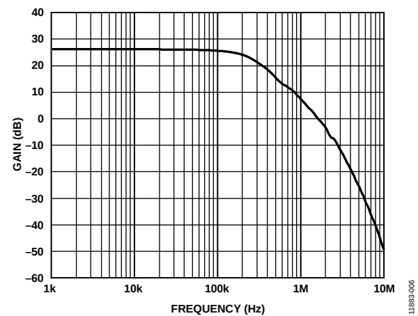
Figure 6. Typical Small Signal Bandwidth ( V_{\text{OUT}} = 200 \text{ mV p-p} )
