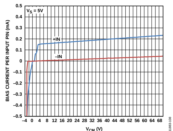
Figure 8. Bias Current per Input Pin vs. Common-Mode Voltage ( V_{\text{CM}} )
