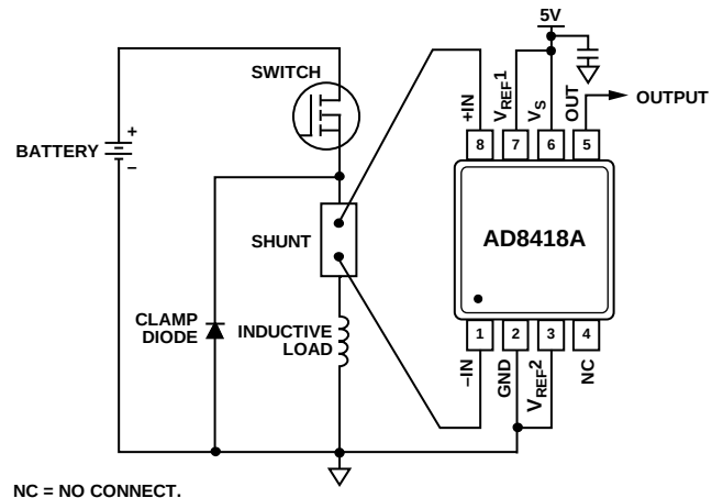
Figure 35. High-Side Switch
