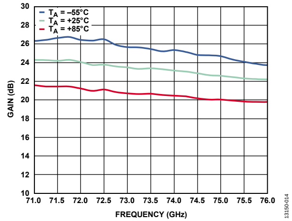
Figure 14. Gain vs. Frequency at Various Temperatures, V_{CTL1}/V_{CTL2} = -5 V
