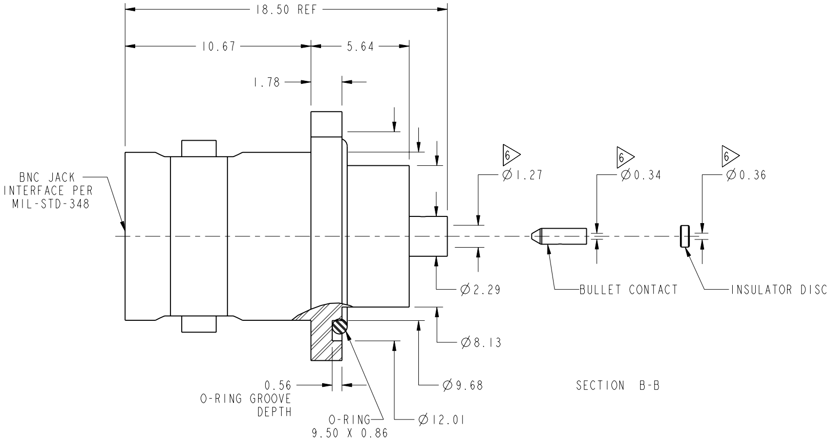
CUSTOMER OUTLINE DRAWING
