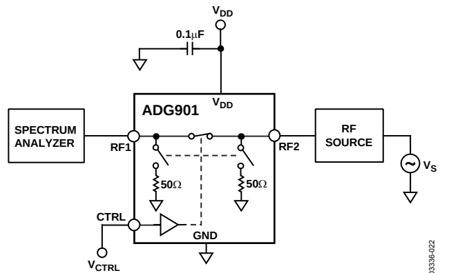
Figure 22. P_{-1dB}
