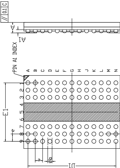
BOTTOM VIEW
