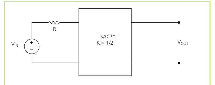
Figure 14 — K = 1/2 Sine Amplitude Converter™ with series input resistor
