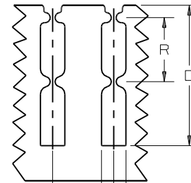
FOR 75mm WALL HGT. 10.0 ± 0.76 [0.39 ± .03] 25.0 ± 0.76 [0.98 ± .03]
