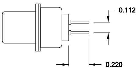
SIGNAL CONTACTS
