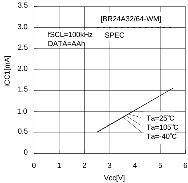
Figure 11. Current consumption at WRITE operation ICC1 ( f_{SCL}=100kHz )
