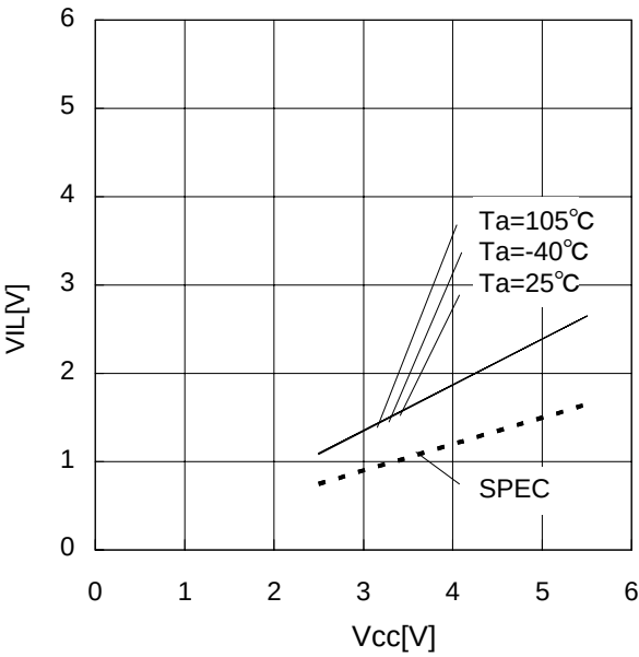
Figure 3. L input voltage V_{IL1,2} (SCL,SDA,WP)
