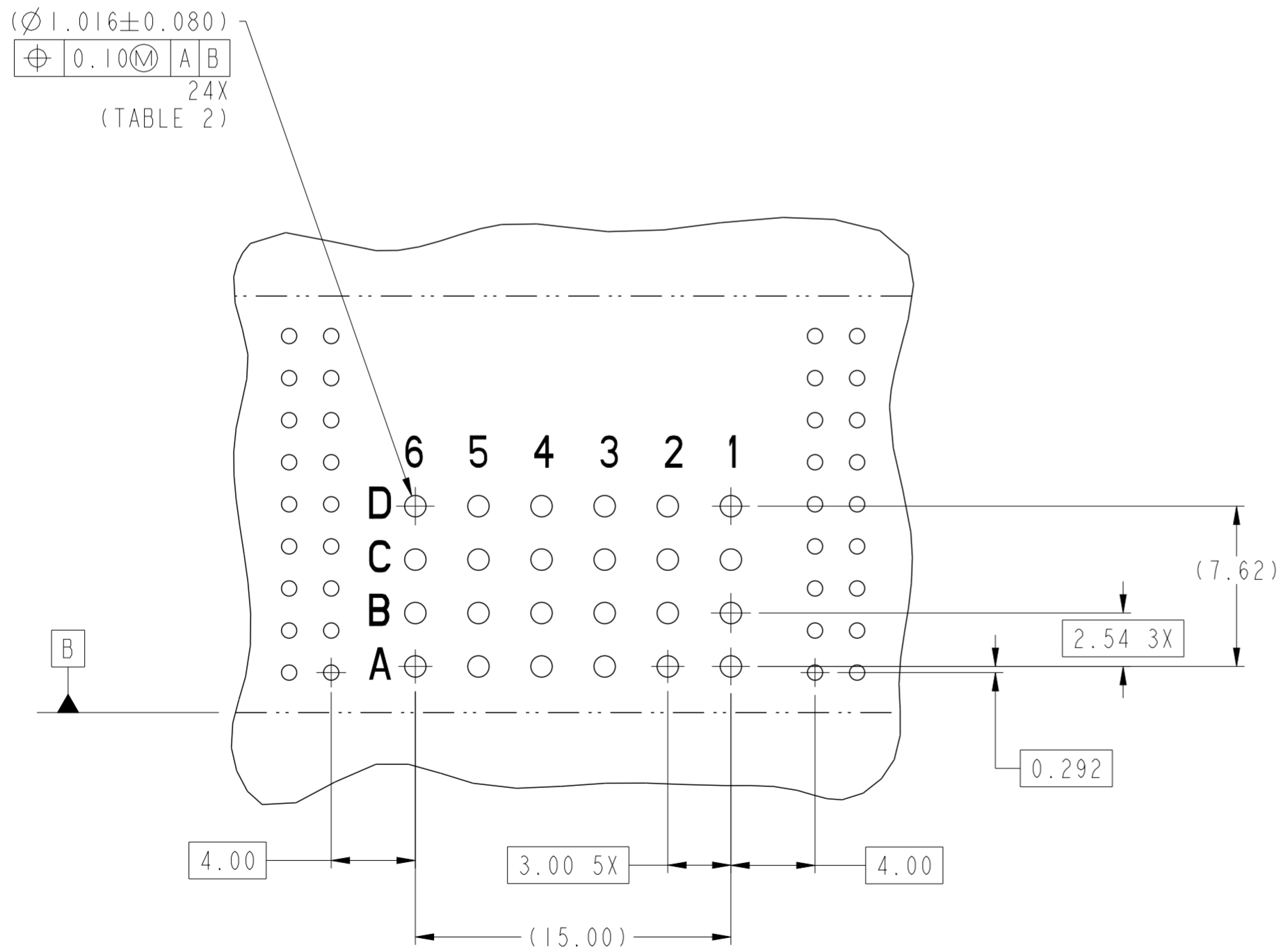
DETAIL E SCALE 4:1
