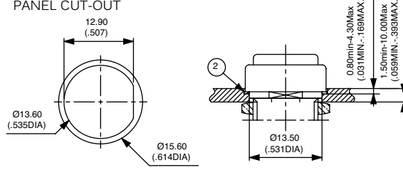
② - O-ring
