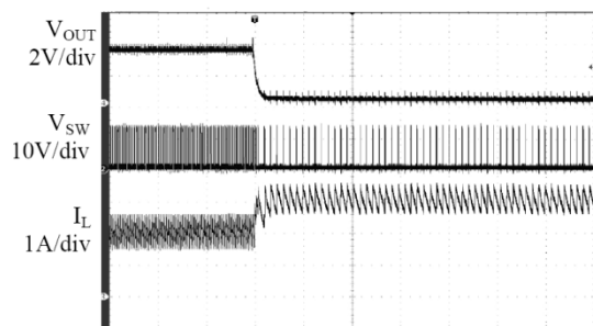
Fig. 14: Short-circuit protection, I_{OUT}=2A
