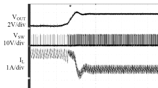
Fig. 15: Short-circuit recovery, I_{OUT}=2A
