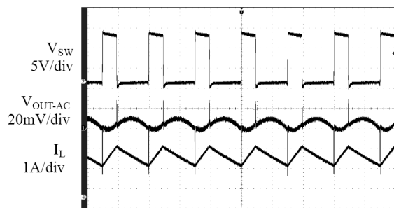
Fig. 10: Output voltage ripple, I_{OUT}=2A
