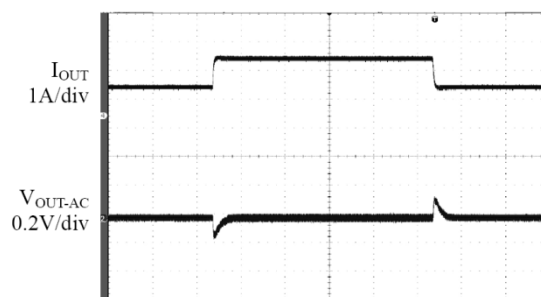
Fig. 11: Load transient ( I_{OUT}=1A to 2A )
