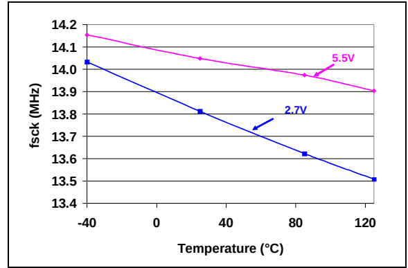
FIGURE 2-53: SCK Input Frequency vs. Voltage and Temperature.
