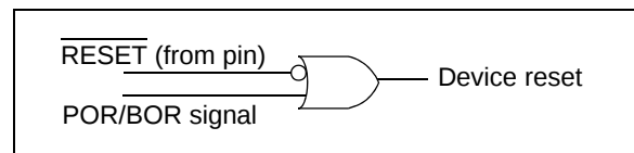
FIGURE 4-1: POR/BOR Signal and \overline{RESET} Pin Interaction.
