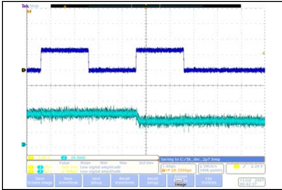
FIGURE 2-12: 5 kΩ – Low-Voltage Decrement Wiper Settling Time ( V_{DD} = 2.7\text{V} ) ( 1\text{ }\mu\text{s/Div} ).
