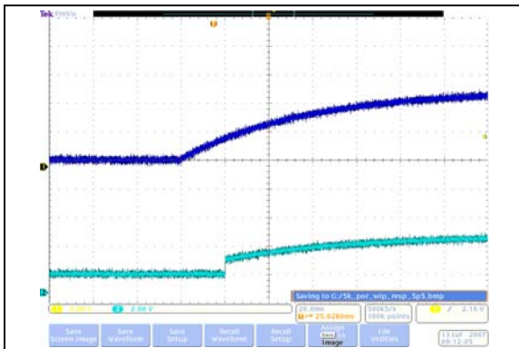
FIGURE 2-14: 5 kΩ – Power-Up Wiper Response Time ( 20\text{ ms/Div} ).
