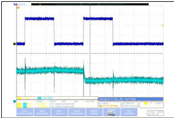
FIGURE 2-13: 5 kΩ – Low-Voltage Decrement Wiper Settling Time ( V_{DD} = 5.5\text{V} ) ( 1\text{ }\mu\text{s/Div} ).
