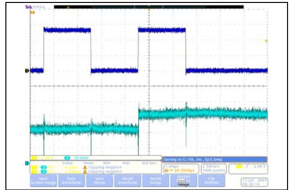
FIGURE 2-16: 5 kΩ – Low-Voltage Increment Wiper Settling Time ( V_{DD} = 5.5\text{V} ) ( 1\text{ }\mu\text{s/Div} ).
