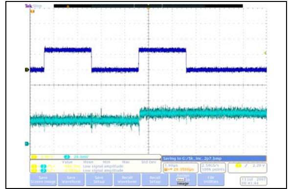
FIGURE 2-15: 5 kΩ – Low-Voltage Increment Wiper Settling Time ( V_{DD} = 2.7\text{V} ) ( 1\text{ }\mu\text{s/Div} ).
