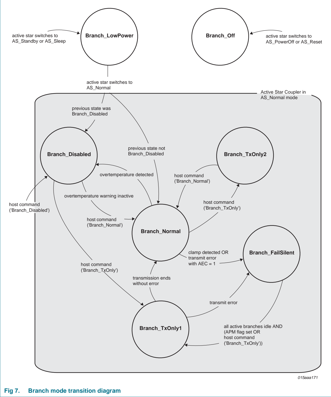
6.9.1.8 Branch operating mode transition diagram
