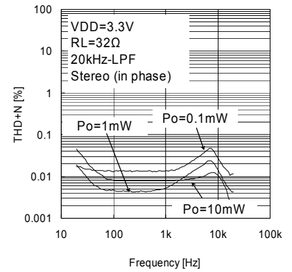
Fig. 46 THD+N vs. Frequency ( VDD=3.3V , RL=32\Omega )
