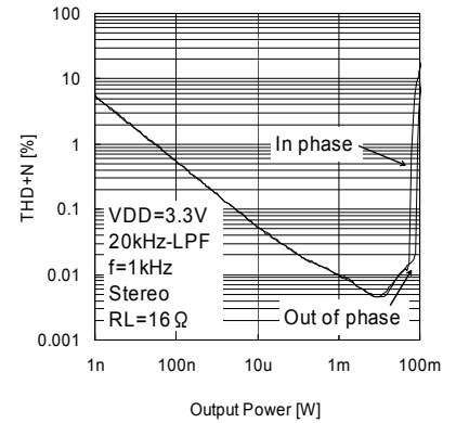
Fig.43 THD+N vs. Output Power ( VDD=3.3V , RL=16\Omega )
