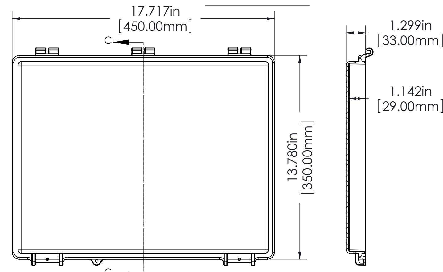
SECTION C-C
