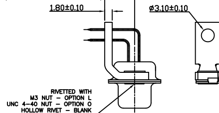
VIEW WITH RIVET &amp; METAL BRACKET
