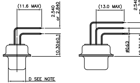
LAYOUT OF 50 POS. CONNECTOR
