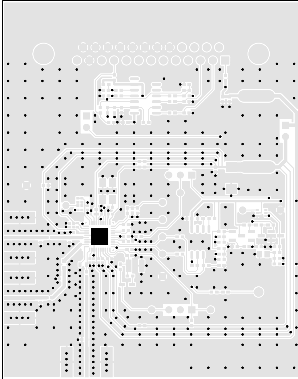
Figure 3. MAX2170 EV Kit PCB Layout—Component Side
