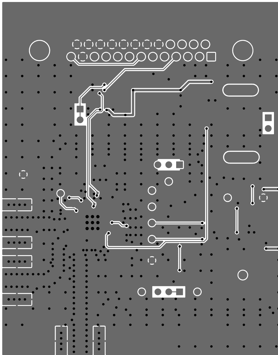
Figure 4. MAX2170 EV Kit PCB Layout—Solder Side
