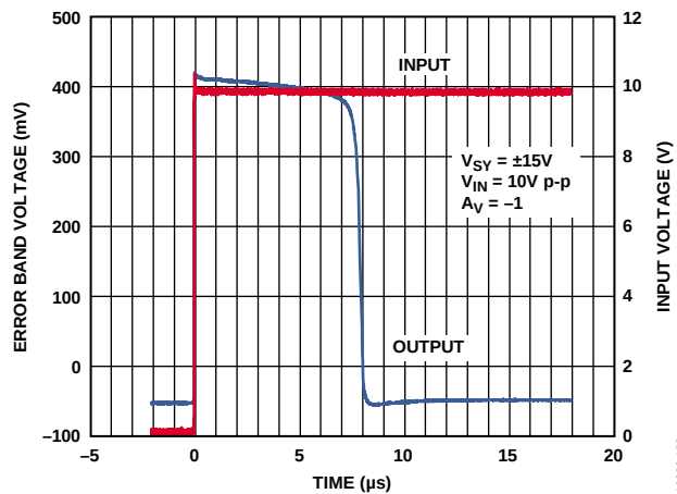
Figure 52. Positive Settling Time
