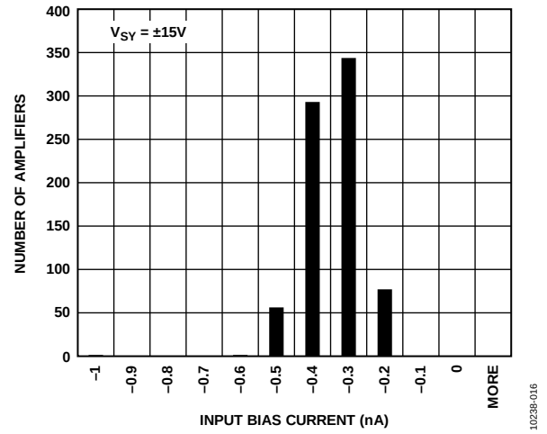
Figure 21. Input Bias Current
