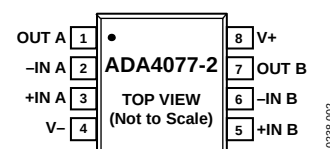
Figure 2. ADA4077-2 Pin Configuration, 8-Lead SOIC_N
