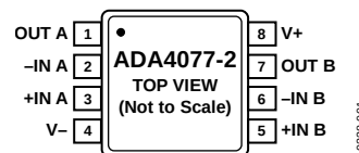
Figure 1. ADA4077-2 Pin Configuration, 8-Lead MSOP
