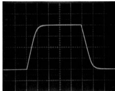
Large Signal Transient Response G = 100, VS = ±15V
