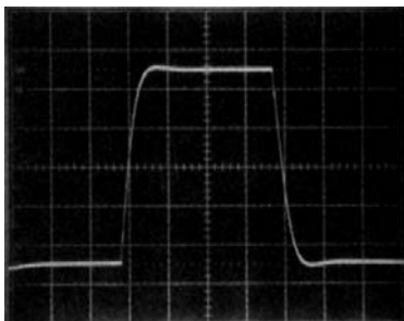
Small Signal Transient Response G = 10, VS = ±15V
