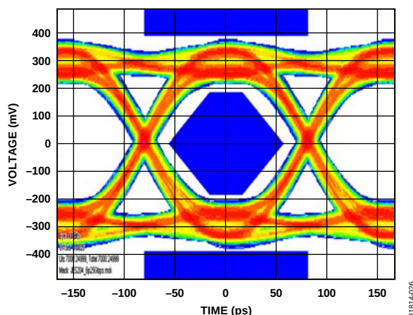
Figure 91. Recovered Data Eye of JESD204B Lane at 6.25 Gbps
