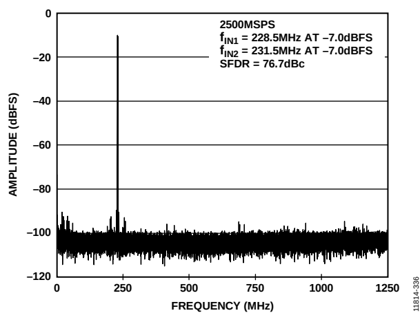
Figure 43. Two Tone FFT Plot at 2.5 GSPS, f_{IN1} = 228.5\text{ MHz} and f_{IN2} = 231.5\text{ MHz} at AIN, -7.0\text{ dBFS} ( \text{SFDR} = 76.7\text{ dBc} )
