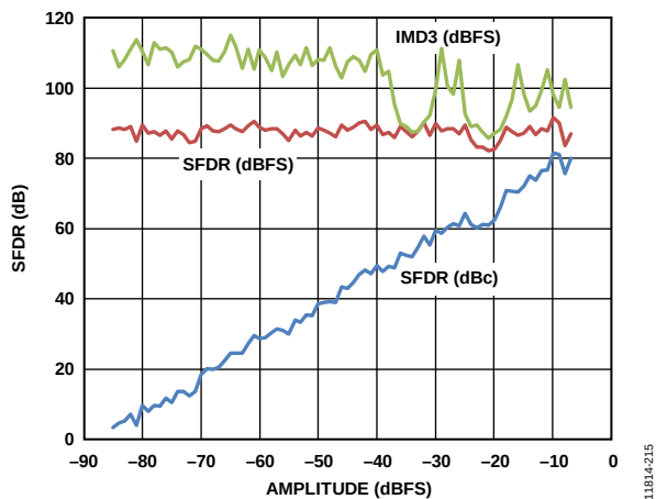
Figure 17. Two Tone SFDR and IMD3 vs. Analog Input Amplitude at 2.0 GSPS at 230 MHz AIN
