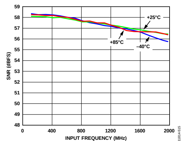
Figure 50. SNR vs. Temperature at 2.6 GSPS
