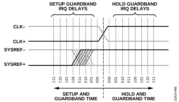
Figure 101. \text{SYSREF} \pm Edge Changes Phase Relative to the Encode Clock, Which can be Detected When the Edge Crosses Through the Guardband Setup Time
