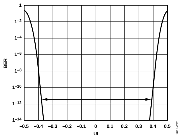
Figure 92. Bathtub Plot of JESD204B Output at 6.25 Gbps
