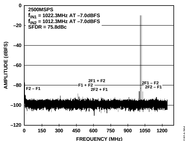
Figure 78. Measured Two-Tone Performance of the Circuit Shown in Figure 80 for a 1 GHz input Signal Using Maximum Gain (15 dB)
