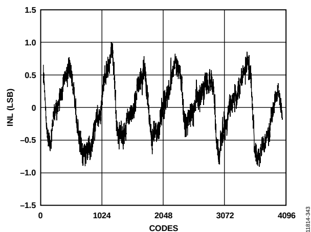
Figure 44. Integral Nonlinearity (INL), \pm 1.0\text{ LSB} at 2.5 GSPS
