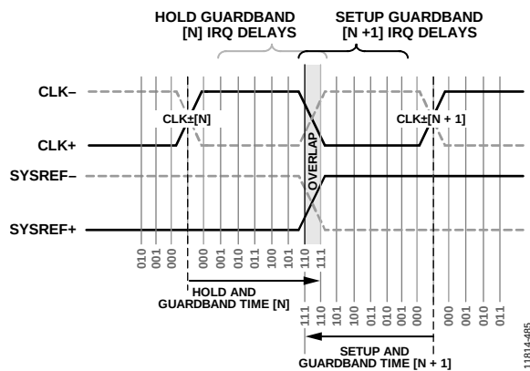
Figure 100. \text{SYSREF} \pm Edge Falls Within Both the Latest Hold Time Guardband of \text{CLK} \pm [N] and the Earliest Setup Time Guardband of \text{CLK} \pm [N + 1] and Triggers an IRQ Error
