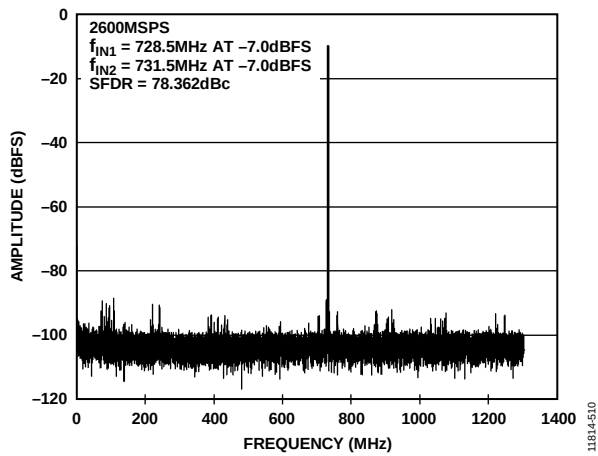
Figure 57. Two Tone FFT Plot at 2.6 GSPS AIN = 730 MHz
