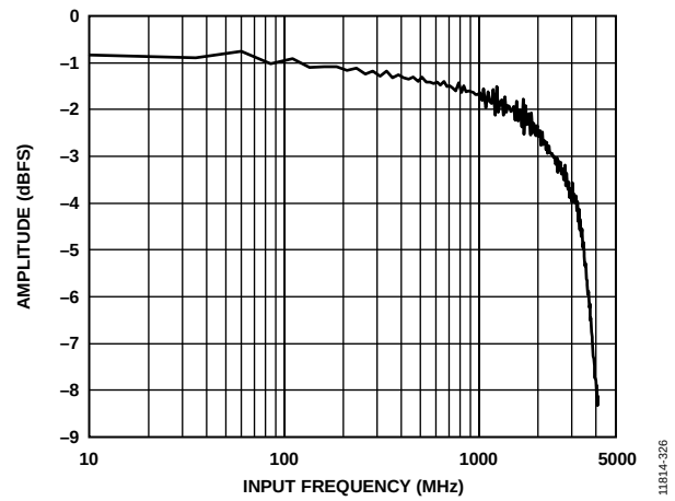
Figure 8. Full Power Input Bandwidth (Input Network in Figure 76 Used &gt;2 GHz, Input Network in Figure 75 Used &lt;2 GHz)
