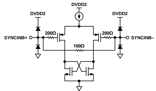
Figure 68. Equivalent SYNCINB± Input
