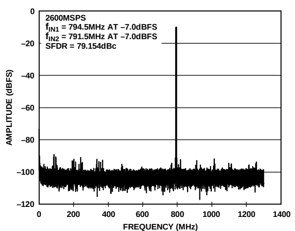
Figure 56. Two Tone FFT Plot at 2.6 GSPS AIN = 1807 MHz
