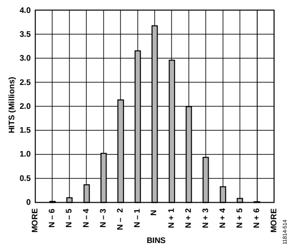
Figure 55. Input Referred Noise Histogram with 2.6 GSPS
