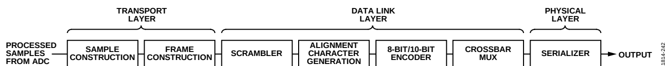
Figure 87. Data Flow
