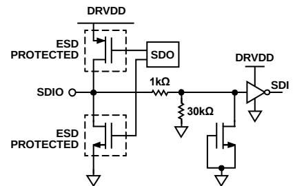
Figure 69. Equivalent SDIO Circuit
