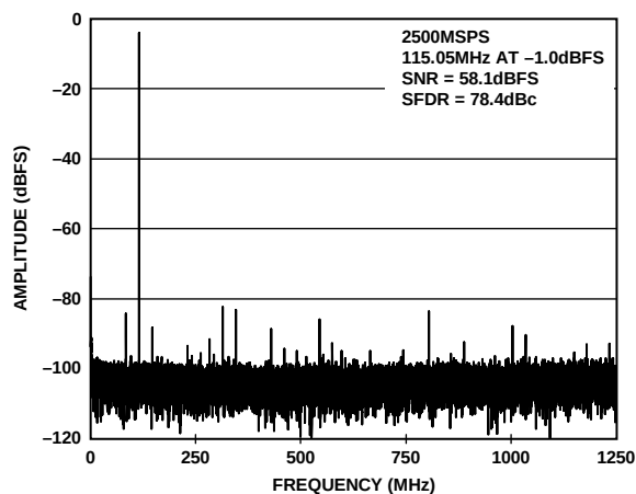
Figure 27. FFT Plot at 2.5 GSPS, f_{IN} = 115.05 MHz at AIN (SFDR = 78.4 dBc, SNR = 58.1 dBFS)
