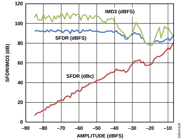
Figure 54. Two Tone SFDR and IMD3 vs. Analog Input Amplitude at 2.6 GSPS at 1807 MHz AIN
