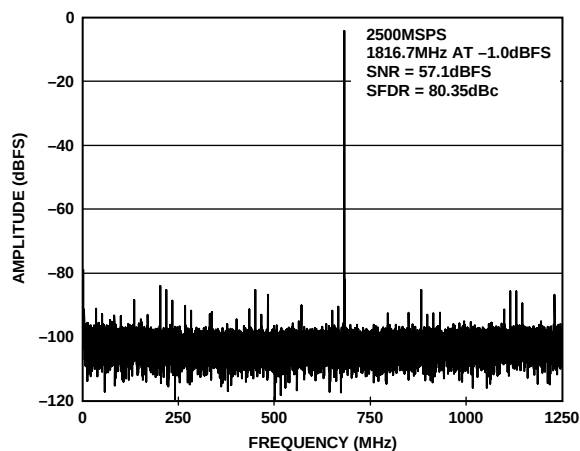
Figure 25. FFT Plot at 2.5 GSPS, f_{IN} = 1816.7 MHz at AIN (SFDR = 80.35 dBc, SNR = 57.1 dBFS)
