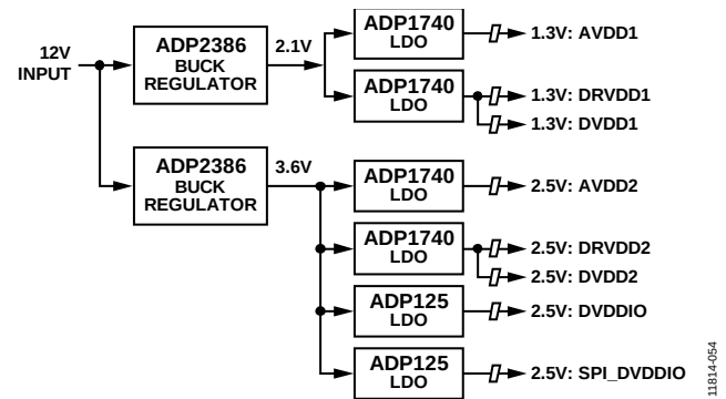
Figure 106. Power Supply Recommendation
