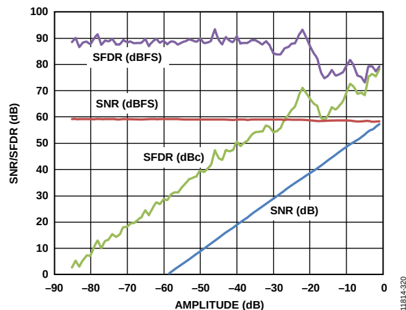
Figure 30. SNR/SFDR vs. Analog Input Amplitude at 2.5 GSPS, f_{IN} = 241 MHz at AIN
