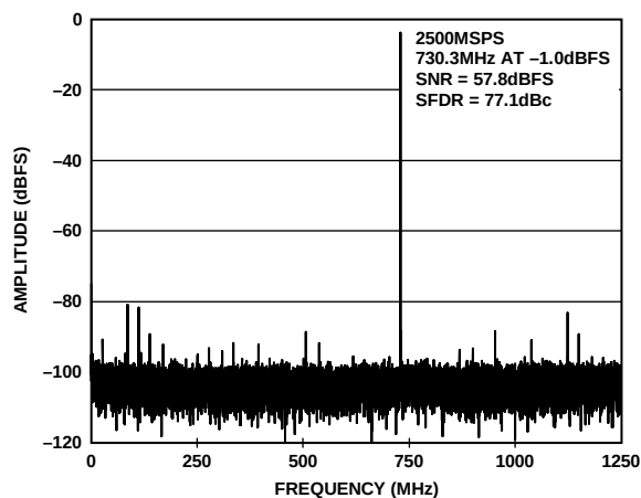
Figure 26. FFT Plot at 2.5 GSPS, f_{IN} = 730.3 MHz at AIN (SFDR = 77.1 dBc, SNR = 57.8 dBFS)
