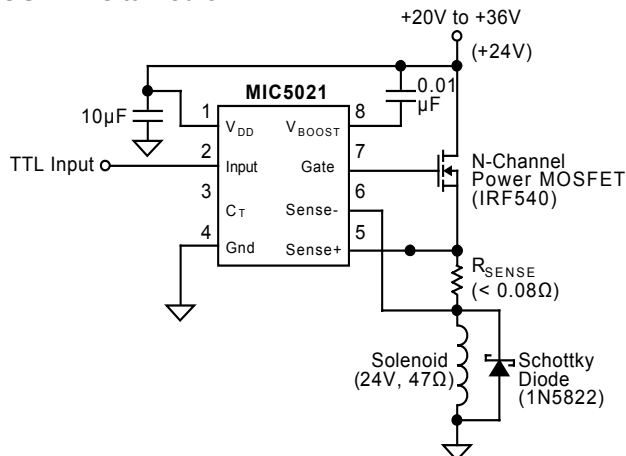
Figure 5. Solenoid Driver with Current Sensing
