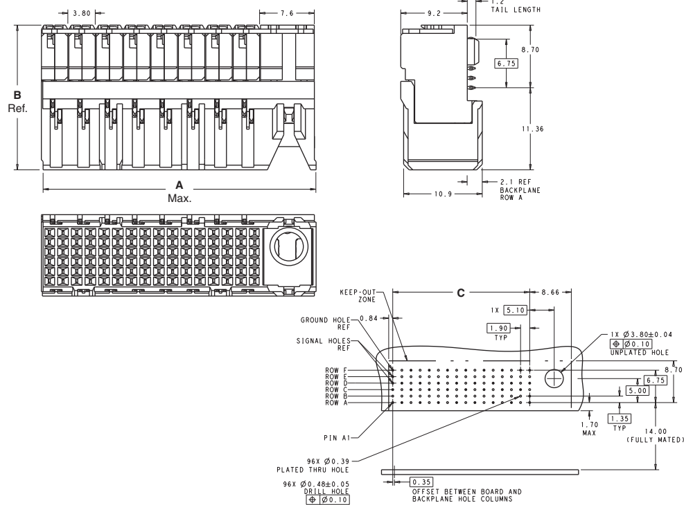
Recommended PCB Layout Min. Board Thickness 1.6
