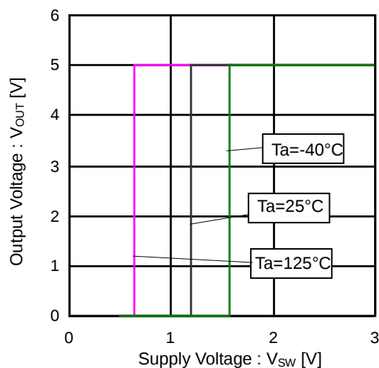
Figure 8. Output Voltage vs SW Input Voltage
