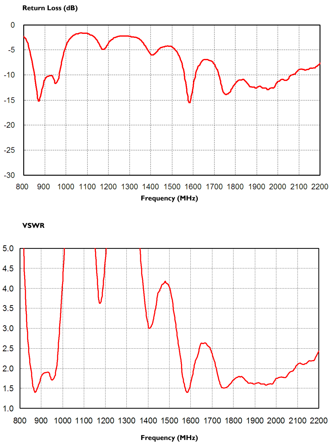
Fig. 3 Return loss &amp; VSWR Measurement
