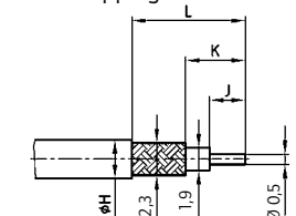
Wire stripping
