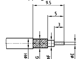
Wire stripping
