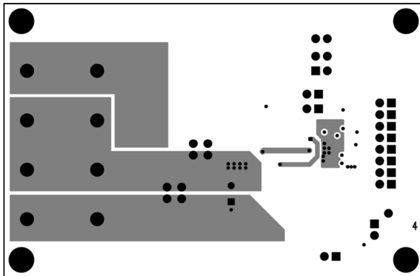
Figure 13. MIC2165 10A Evaluation Board Bottom Layer
