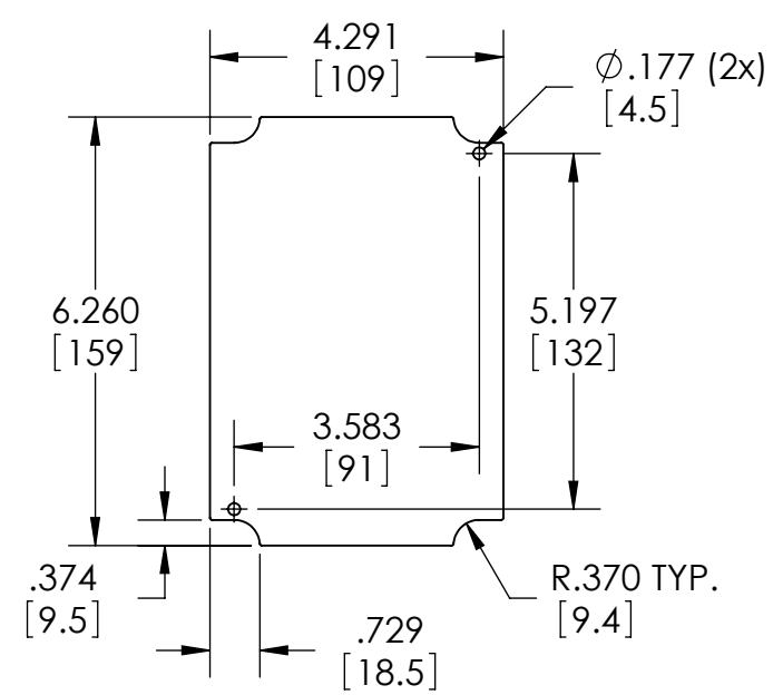
SUGGESTED PC BOARD LAYOUT
