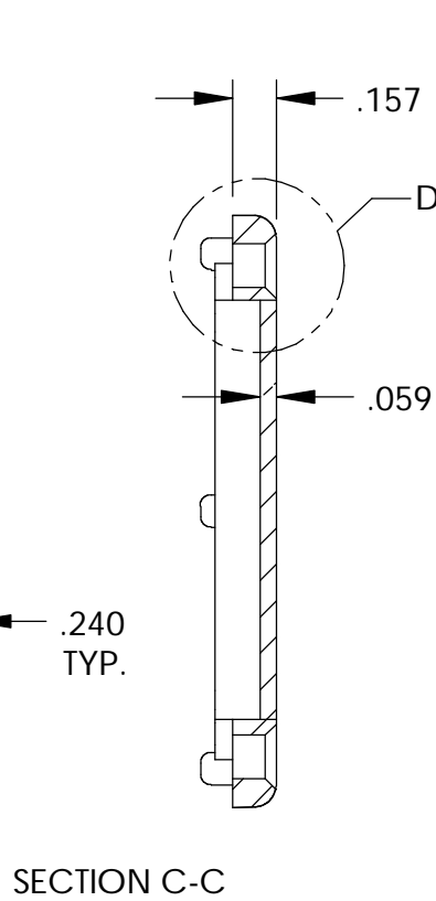
SECTION C-C
