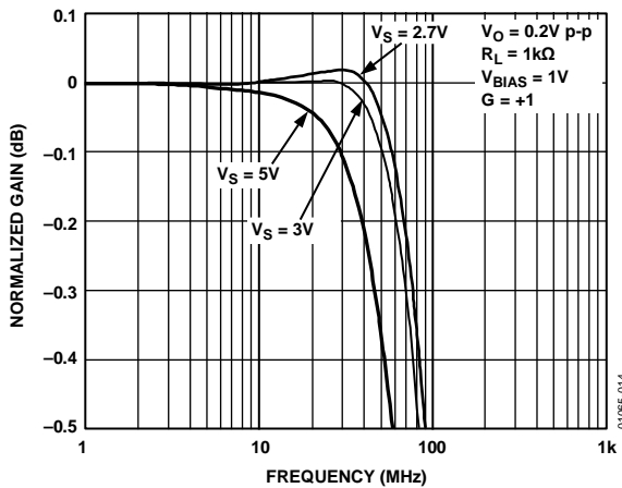
Figure 14. 0.1 dB Flatness
