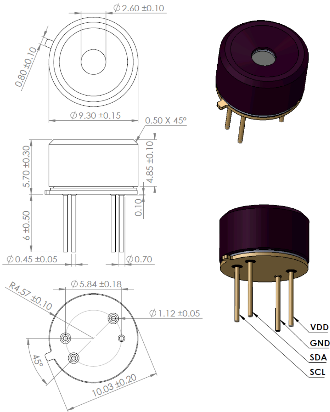
Figure 30 Mechanical drawing of 110° FOV device
