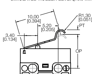
TYPE G SIMULATED ROLLER LEVER (10,0 mm, R1,3)
