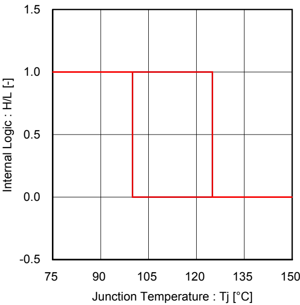
Figure 43. Thermal Shutdown
