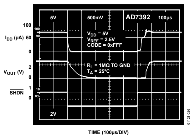
Figure 23. Shutdown Recovery Time
