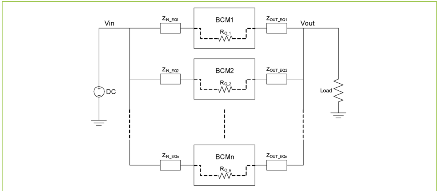
Figure 17 – BCM Array
