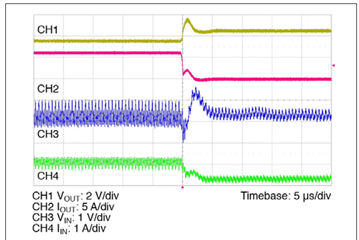
Figure 12 – Negative load transient (7.7 A – 0 A)
